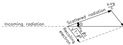
FIGURE 6.3.1. Compton scattering
